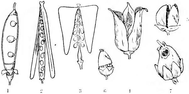
DEHISCENT FRUITS
